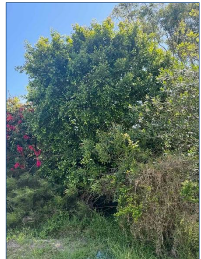
Figure 6: Tree 4.
