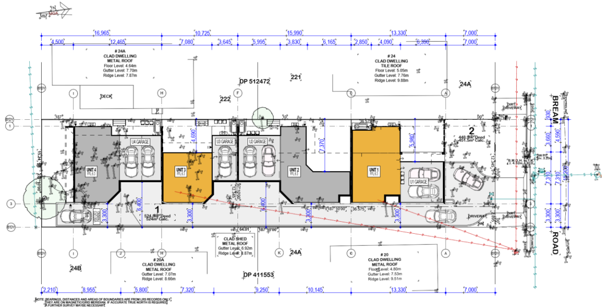
Figure 4: Extract of the site plan of the development.
