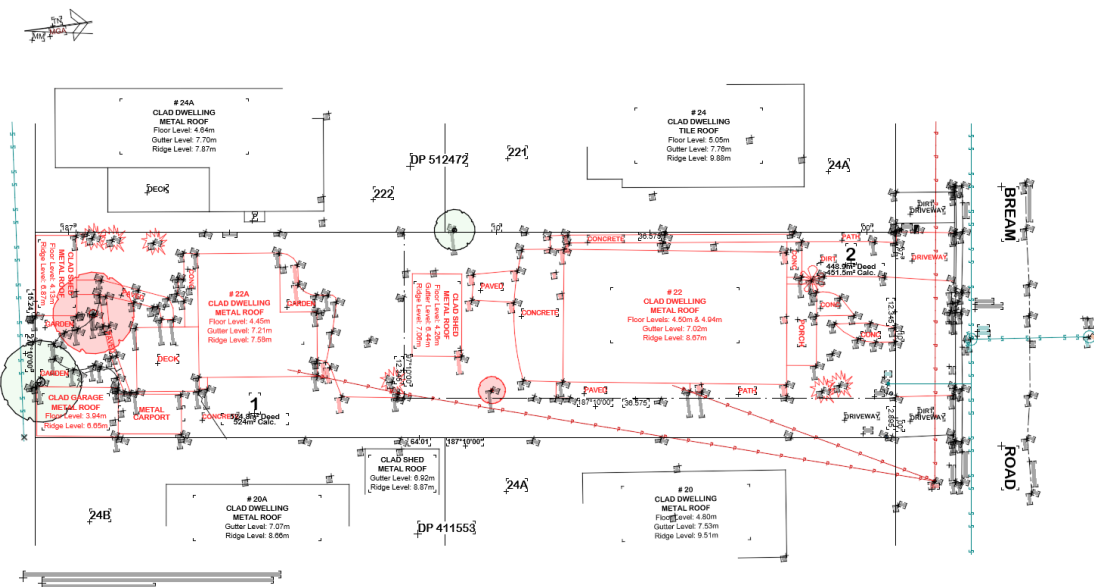
Figure 5: Extract of the demolition plan of the development.
