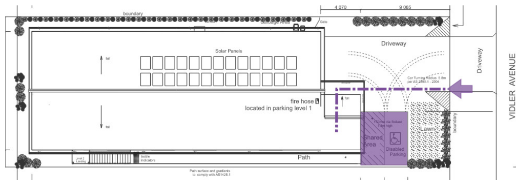
Figure 2 | Overall Site Plan
